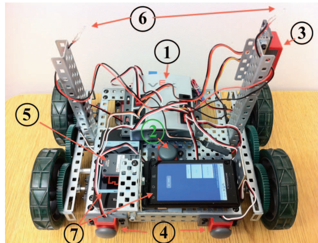
Figure 1. Phone Robot Hybrid: 1- VEX Microcontroller, 2 - Start button, 3 - Ultrasonic Range Finder, 4 - Front bumpers, 5 - Light Sensor, 6 - LED's used for debugging, 7 - iPhone 4 and Motorola Droid.
